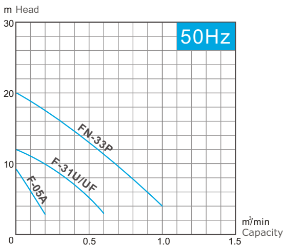
Non-clogging Impeller
